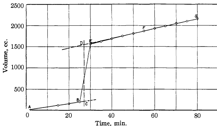
Fig. 4.—Volume-time curve for determination No. 4 on N_2O_5 .
