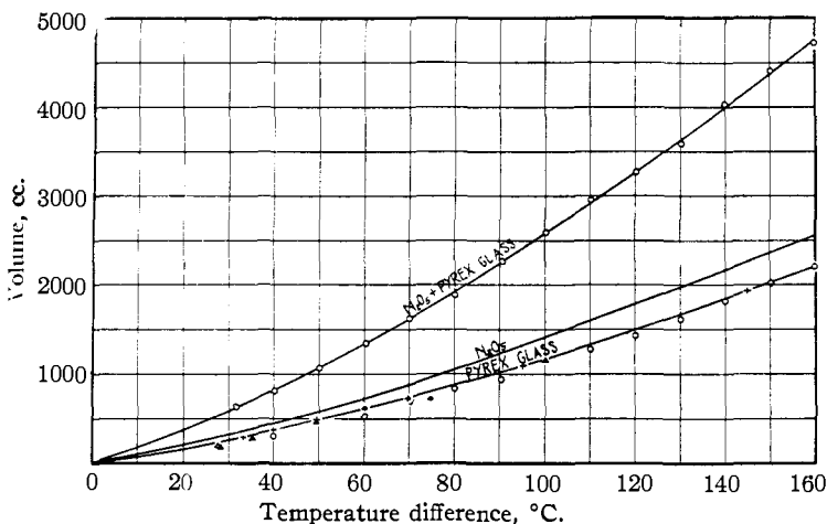
Fig. 5.— \Delta V-\Delta T curve for N_2O_5 .
