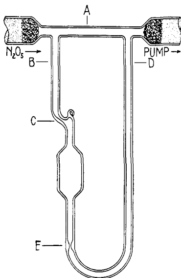
Fig. 3.—Arrangement of dropping-bulb in N_2O_5 distillation apparatus.
