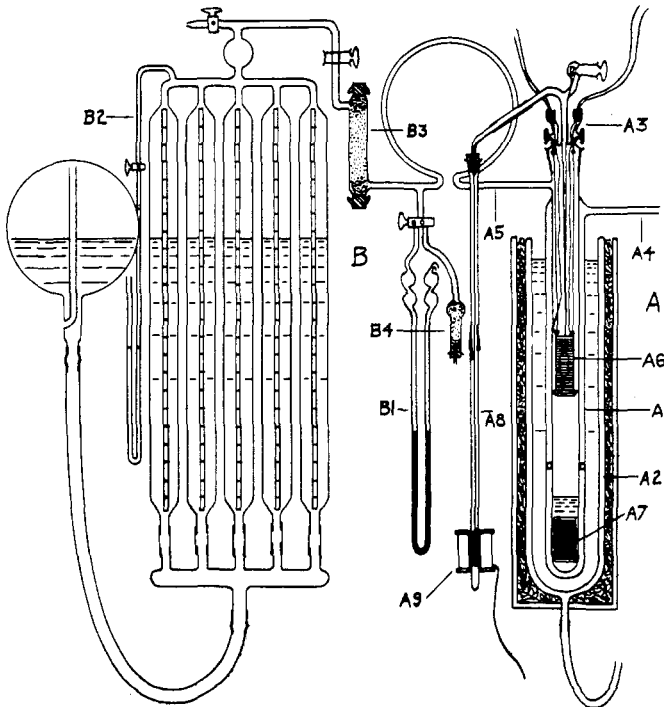
Fig. 1.—Assembly of apparatus.
